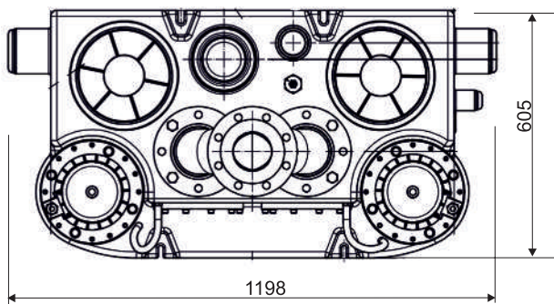
Assembly example for estimating the space requirement of the lifting unit
